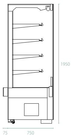
SECTION ELEVATION
