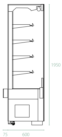
SECTION ELEVATION
